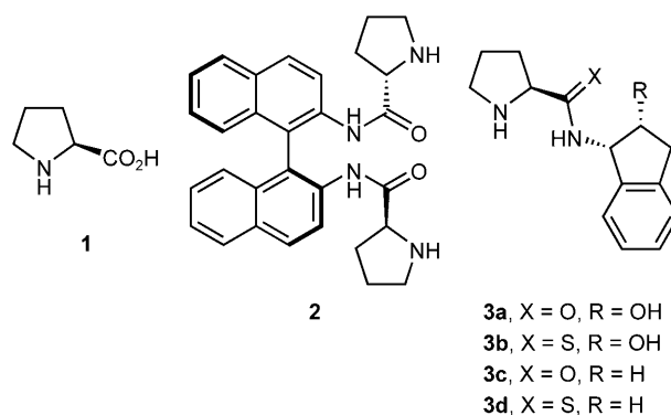
Figure 1. Organocatalysts for the direct solvent-free aldol reaction.
