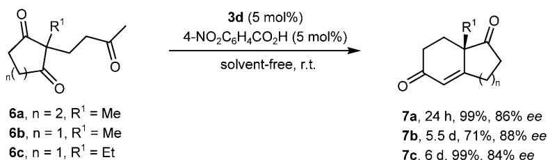
Scheme 2. Intramolecular solvent-free aldol reactions catalyzed by 3d .
