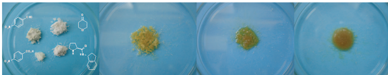
Figure 2. Aldol reaction of tetrahydro-4 H -thiopyran-4-one with 4-nitrobenzaldehyde catalyzed by 3d (30 mol%)/4-NO 2 C 6 H 4 CO 2 H (30 mol%) after 1 h (left center), 2 h (right center), and 5 h (right) at room temperature without stirring.
