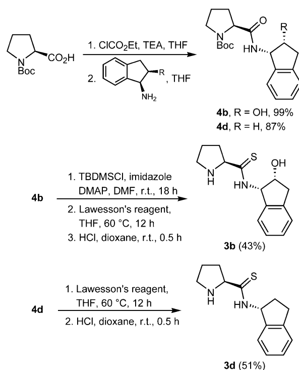
Scheme 1. Synthesis of prolinethioamides 3b and 3d .
